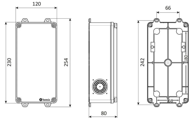
TECHNICAL DRAWING
