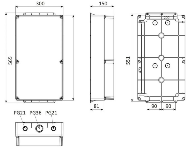
TECHNICAL DRAWING
