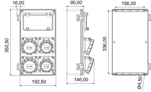
TECHNICAL DRAWING
