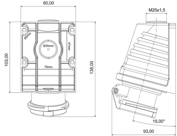
TECHNICAL DRAWING
