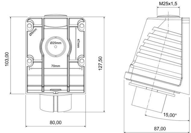
TECHNICAL DRAWING
