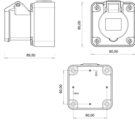
TECHNICAL DRAWING
