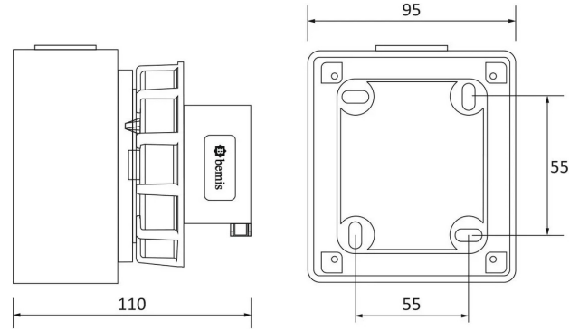
TECHNICAL DRAWING
