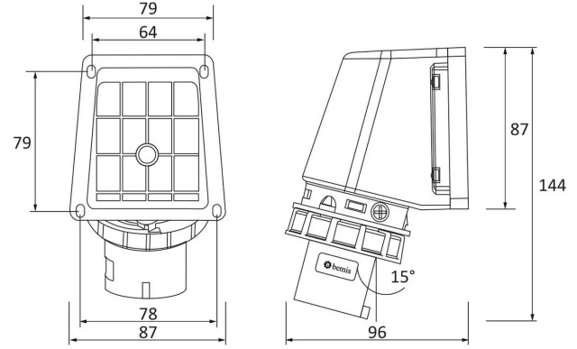
TECHNICAL DRAWING
