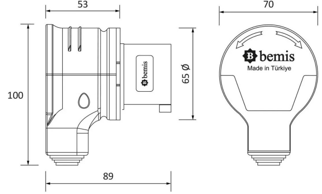
TECHNICAL DRAWING
