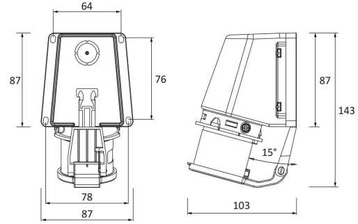
TECHNICAL DRAWING
