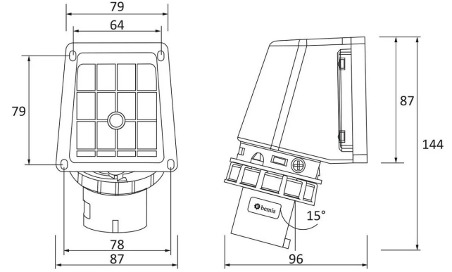
TECHNICAL DRAWING
