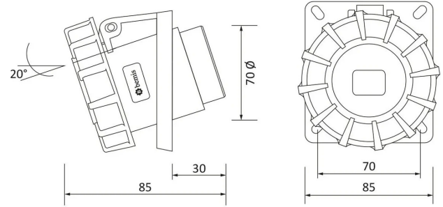
TECHNICAL DRAWING
