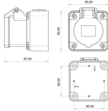
TECHNICAL DRAWING
