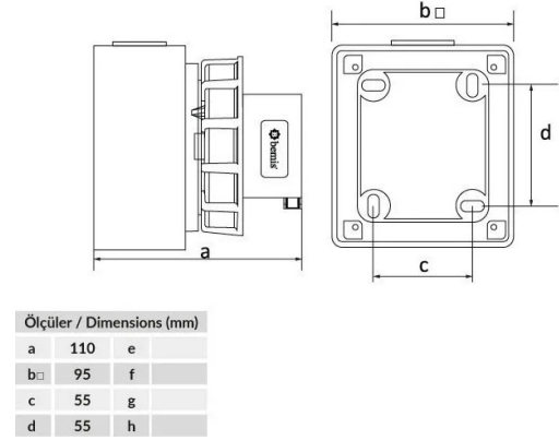
TECHNICAL DRAWING
