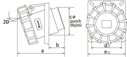
TECHNICAL DRAWING
