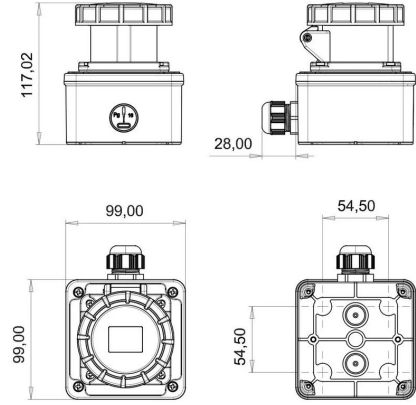
TECHNICAL DRAWING
