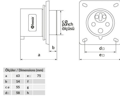
TECHNICAL DRAWING
