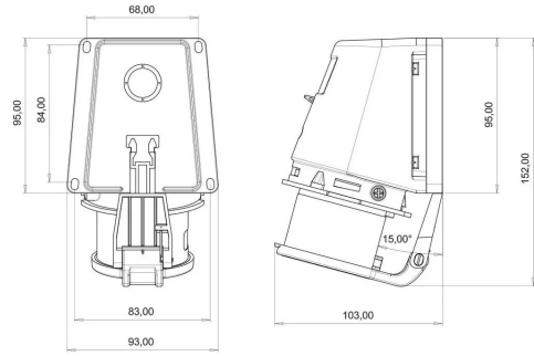
TECHNICAL DRAWING
