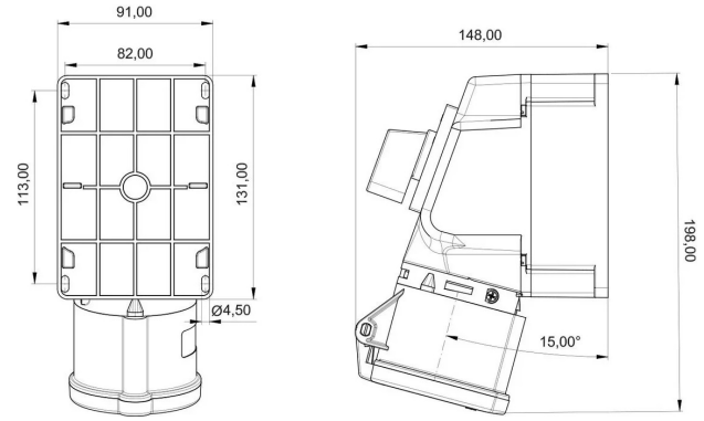
TECHNICAL DRAWING
