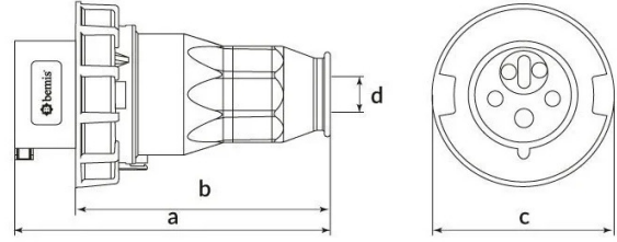
TECHNICAL DRAWING
