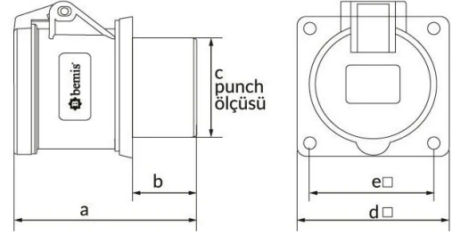
TECHNICAL DRAWING
