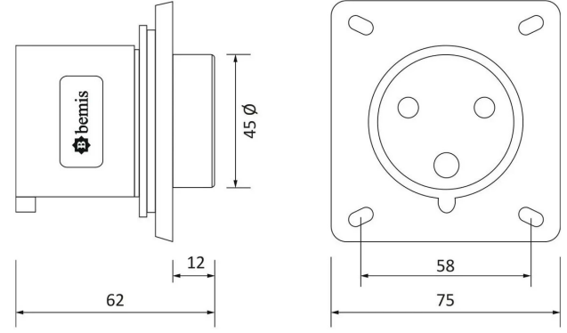
TECHNICAL DRAWING
