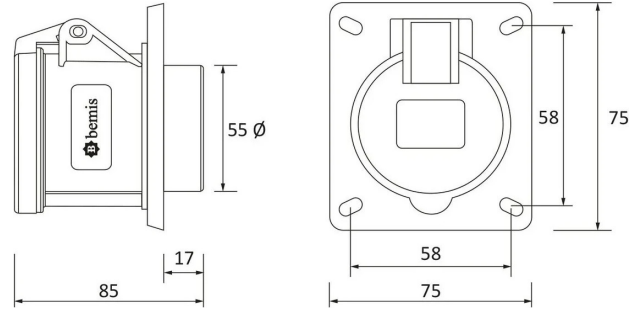
TECHNICAL DRAWING
