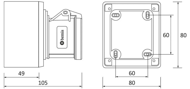
TECHNICAL DRAWING
