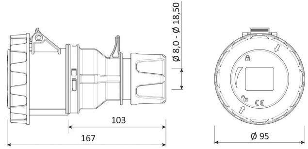
TECHNICAL DRAWING
