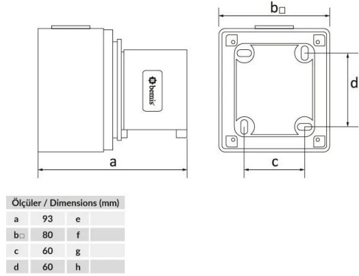
TECHNICAL DRAWING
