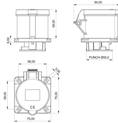
TECHNICAL DRAWING
