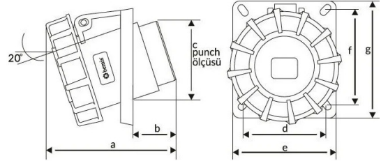
TECHNICAL DRAWING
