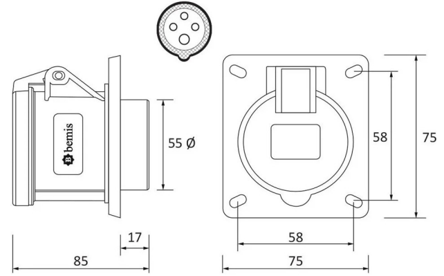
TECHNICAL DRAWING
