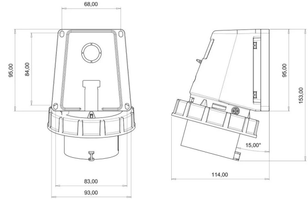
TECHNICAL DRAWING
