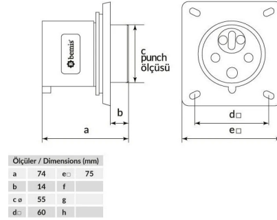
TECHNICAL DRAWING
