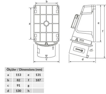
TECHNICAL DRAWING
