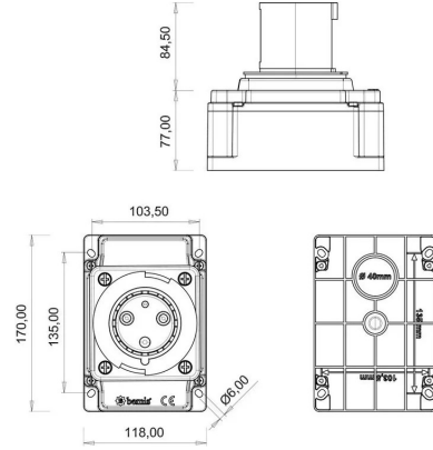
TECHNICAL DRAWING
