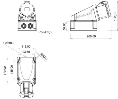
TECHNICAL DRAWING
