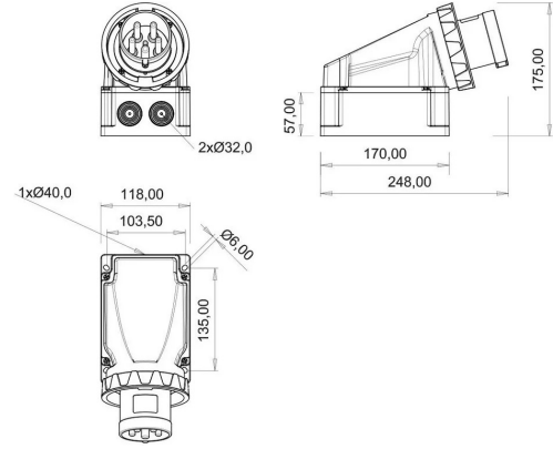
TECHNICAL DRAWING
