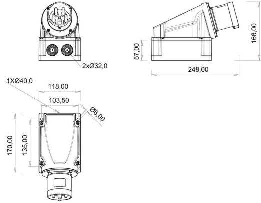
TECHNICAL DRAWING
