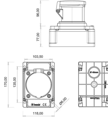
TECHNICAL DRAWING
