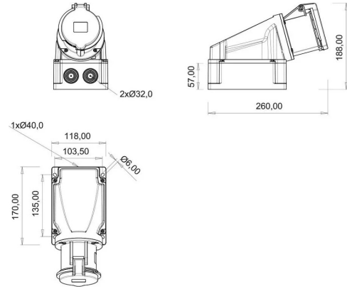
TECHNICAL DRAWING
