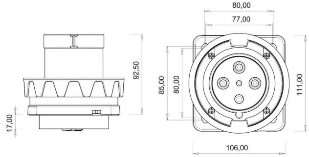
TECHNICAL DRAWING
