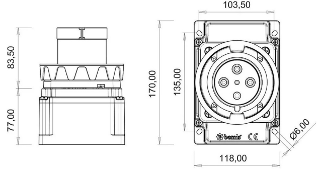
TECHNICAL DRAWING
