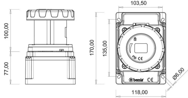
TECHNICAL DRAWING
