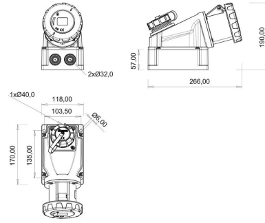
TECHNICAL DRAWING
