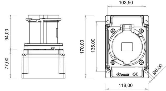
TECHNICAL DRAWING
