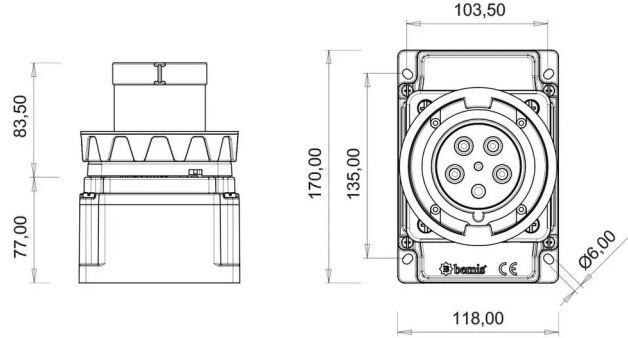
TECHNICAL DRAWING
