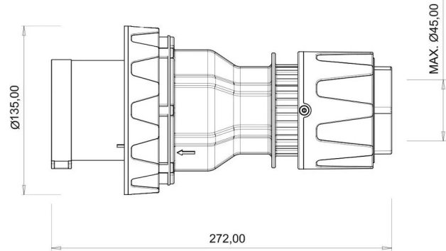
TECHNICAL DRAWING
