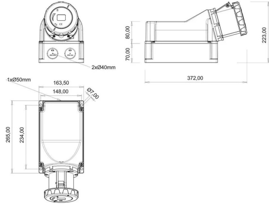
TECHNICAL DRAWING
