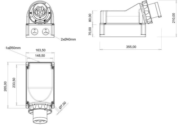
TECHNICAL DRAWING
