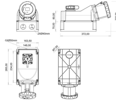
TECHNICAL DRAWING
