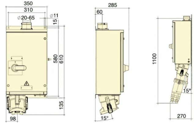
TECHNICAL DRAWING
