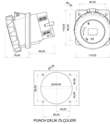
TECHNICAL DRAWING
